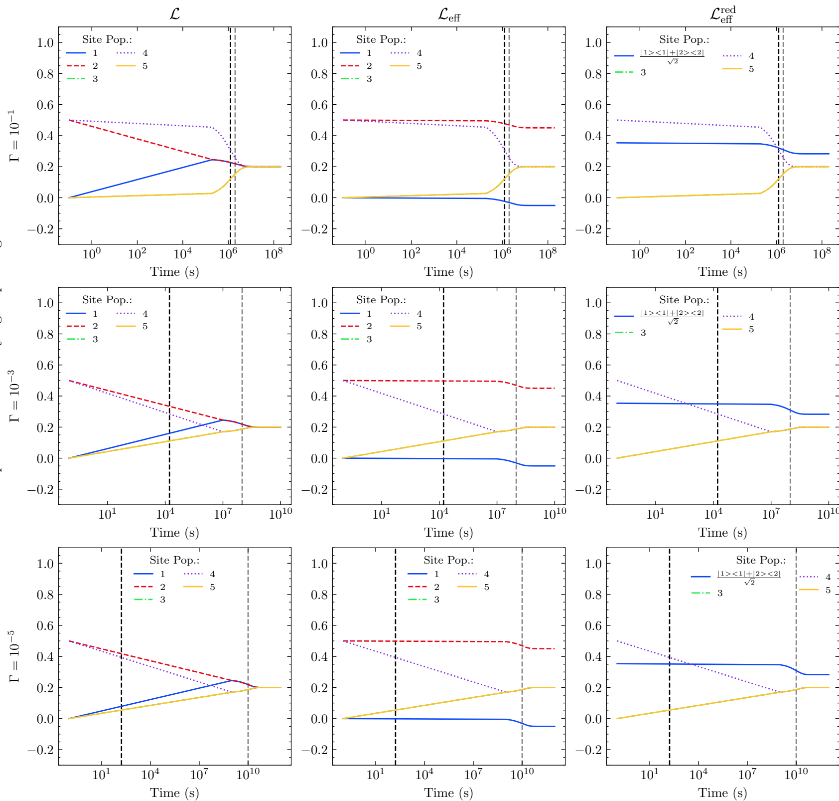
Time Evolution of Site Populations under \mathcal{L} , \mathcal{L}_{\text{eff}} , and \mathcal{L}_{\text{eff}}^{\text{red}} Initially: Site 2 and 4 at 0.5, rest empty N=5 ; J = 10^{-1} ; \epsilon = 10^{-4}
